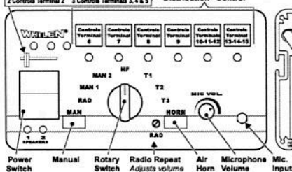
3 Pos. Slide Switch: 3 = OFF 1 Controls Terminal 1 2 Controls Terminal 2 3 Controls Terminals 3, 4 & 5
